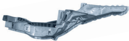
Machining of a side member with downstream Helicoil assembly
